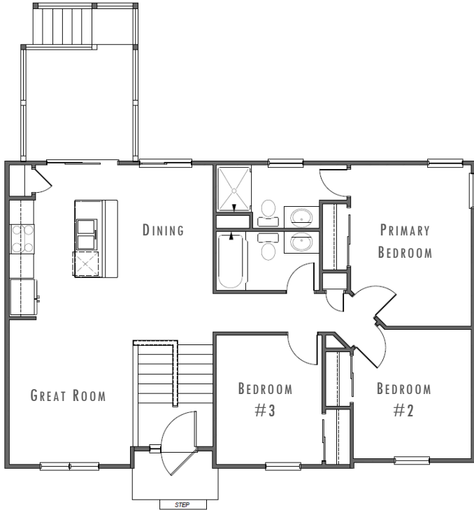
main level
